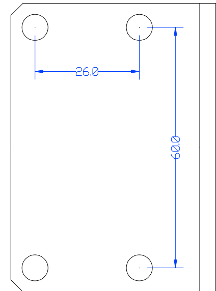
SIDE MOUNTING
